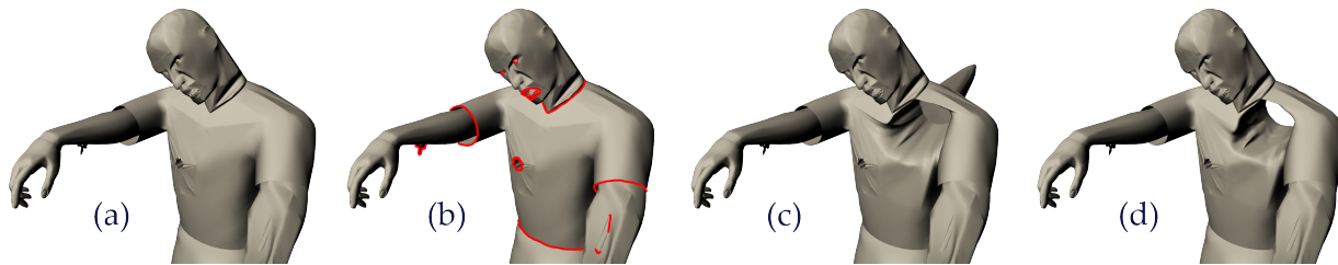
Figure 1: This zombie model (a) has numerous open surfaces, non-manifold edges, and self-intersections, displayed in red here (b). None-the-less, using the technique described in this paper, we are able to (c) poke through the zombie’s chest and (d) create the desired tunnel/hole.
