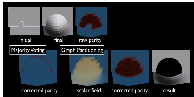
Figure 7: Majority voting works poorly when intersection curves don't separate the surface. Graph partitioning allows us to introduce new cuts into the mesh.
