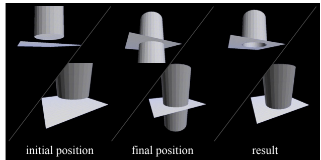
Figure 4: When a cylinder is plunged downwards into a ground plane, our method reacts as depicted. However, methods which only inspect the final position of the mesh are faced with an ambiguously symmetric problem.
