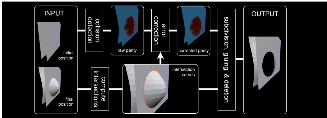
Figure 5: Overview of our method and its components
