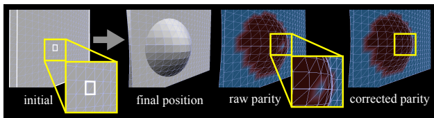
Figure 6: When surfaces have holes (inset, initial) the raw parity field can be corrupted (raw parity, inset). Running error correction removes these isolated errors.
