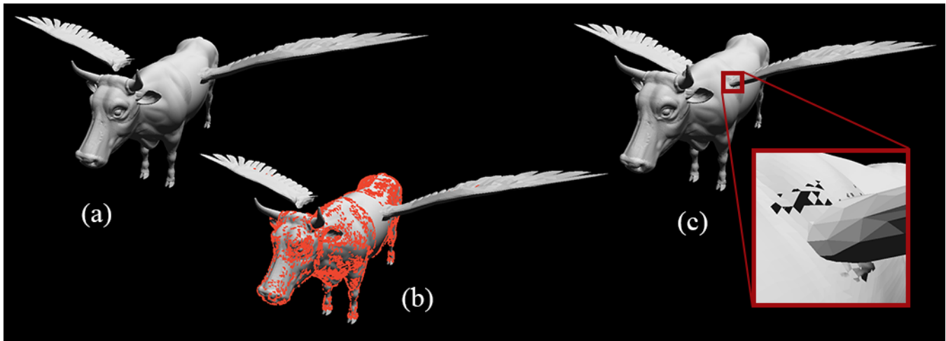
Figure 12: We attach a pair of wings to a cow model (a) composed of many disconnected components, intersecting as shown (b) in red. Nonetheless, we are able to (c) compute topology change. (Inset) Error correction cannot fix completely disconnected components.
