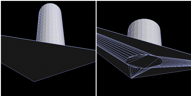
Figure 13: A failure case of our algorithm. A closed cylinder plunges downward through a single giant triangle (left). Because there are no parity samples on the triangle itself, our algorithm does not properly delete the hole caused by the cylinder. Instead, it causes a non-manifold junction between both models (right).
