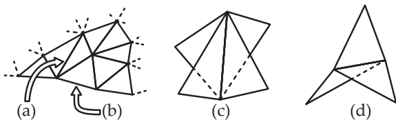
Figure 2: Mesh type locally depends on the number of triangles incident to an edge: (a) manifold edge, (b) boundary edge, (c) closed edge, (d) non-manifold, non-closed, non-boundary edge
